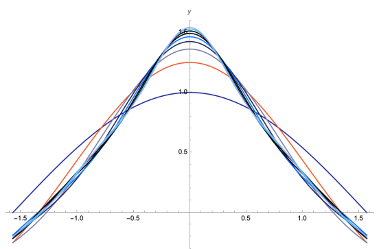
Fig. 8.8: Partial sums s_k = \sum_{n=1}^k \frac{\cos nx}{n^2} for the series \sum_{n=1}^{\infty} \frac{\cos nx}{n^2}
