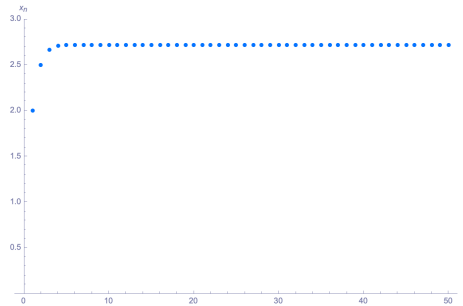
Fig. 3.1: y_n = (1 + \frac{1}{n})^n
